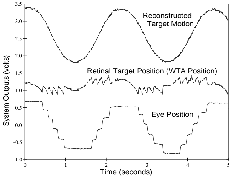
Figure 5: Saccades-only Tracking: In this example, a swinging target consisting of a single edge with no distractors is tracked over a few cycles. The middle trace shows the WTA position voltage which encodes the position of the tracked target on the retina. The bottom trace shows the eye position and the top trace is the reconstructed target motion, computed by adding the retinal position to the eye position. Re-centering saccades are triggered when the target leaves a specified window centered on the array.
