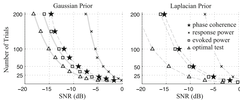
Fig. 3 The number of trials needed to achieve 80 % statistical power at different SNR values, for background activity subject to a Gaussian ( c=2 ) or Laplacian ( c=1 ) distribution. Each point in the figure is a Monte Carlo numerical result. Theoretical values, when known, are plotted as (solid gray lines). Test statistics whose curves lie more to the
