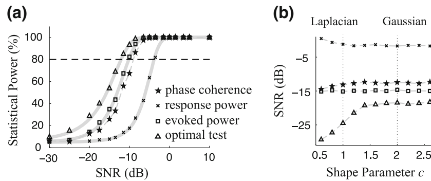
Fig. 2 (a) The statistical power of four significance tests as a function of SNR when background activity is subject to the Gaussian distribution. Each point in the figure is a Monte Carlo numerical result; the theoretical statistical power, when available, is plotted as a (solid gray line). Test statistics whose curves lie more to the left possess greater statistical power at the same SNR than those to the right. Similarly, to achieve 80 % statistical power, each test requires a different minimum
