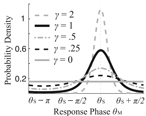
Fig. 1 The probability density function of the phase of neural measurements when stimulus-synchronized activity is generated independently of background activity. The probability distribution is distinct from the uniform distribution (solid gray line), as long as stimulus-synchronized activity has non-zero amplitude
