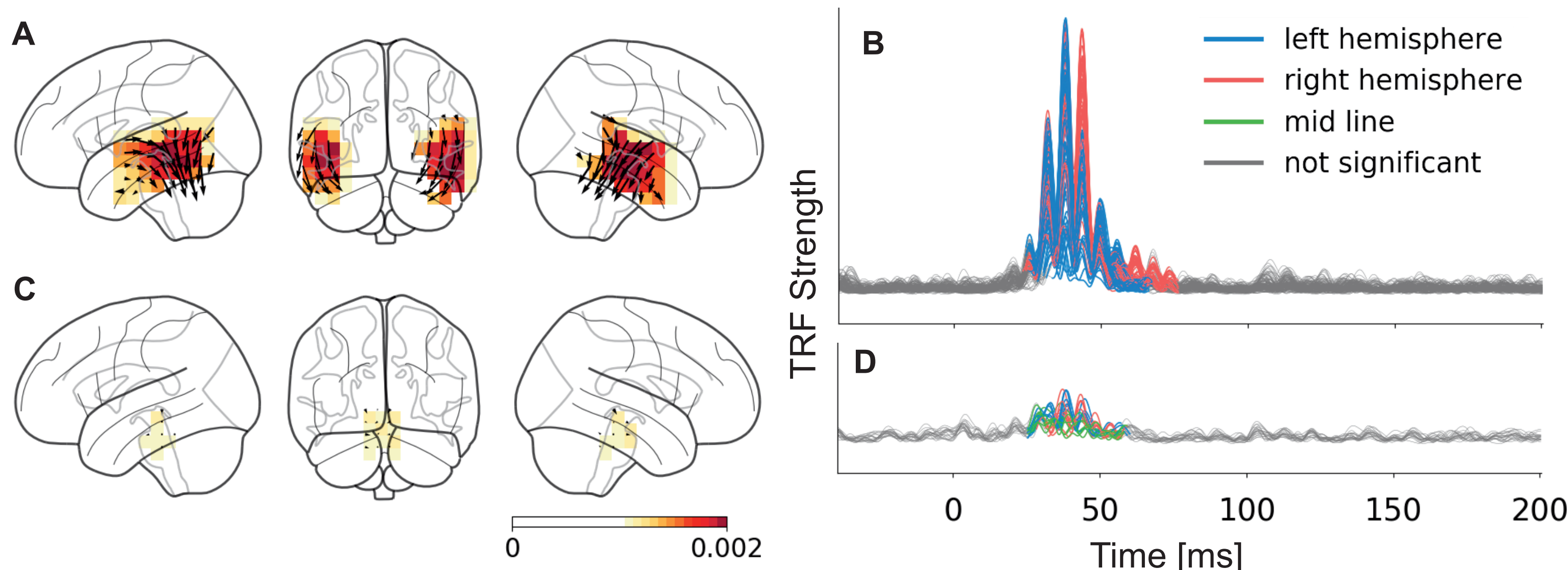
Volume Source Space TRFs: (A) Peak TRF vectors in voxels closest to temporal lobe. (B) TRFs of voxels closest to temporal lobe. (C) Peak TRF vectors of voxels closest to brainstem. (D) TRFs of voxels closest to brainstem. (for the envelope predictor)
