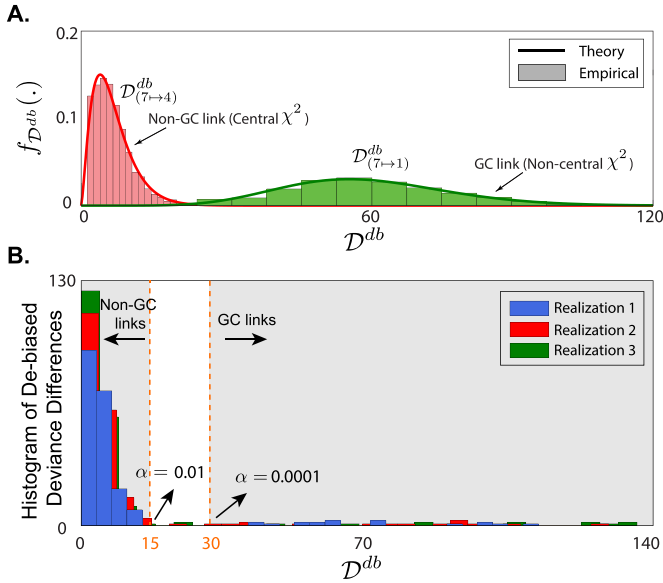
Fig. 3. Empirical validation of Theorem 1 . A. Theoretical and empirical distributions of the de-biased deviance differences corresponding to the GC link ( 7 \rightarrow 1 ) and non-GC link ( 7 \rightarrow 4 ) from the setting of Fig. 2 . The empirical distributions closely match the theoretical predictions of Theorem 1 . B. Histogram of the de-biased deviance differences of all possible links between the first 15 sources for three different realizations of the VAR processes with the same parameters and for two significance levels \alpha = 0.01 and 0.0001 . The de-biased deviance differences show a clear delineation of the significant GC links (to the right of the dashed vertical lines) and insignificant ones (to the left of the dashed vertical lines), while exhibiting robustness to the choice of the significance level.
