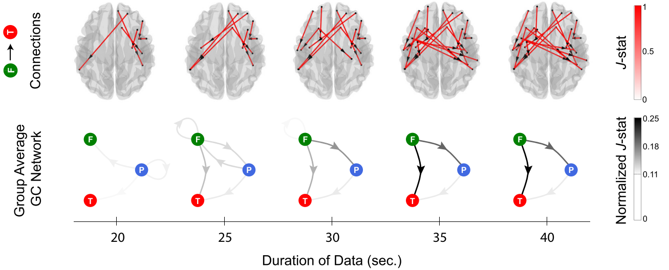
Fig. 12. Evaluating the effect of trial duration on the NLGC performance. The group average GC links from frontal to temporal areas for younger participants during tone processing are overlaid on the dorsal brain plot in the top row. The corresponding directed graphs indicating the normalized J -statistics of the links between frontal, temporal, and parietal areas are shown in the bottom row. Columns correspond to different choices of T corresponding to the first 20, 25, 30, 35 and 40 s of the data. While for smaller values of T , several links are missing, by increasing T beyond 30 s the detected networks stabilize and converge.
