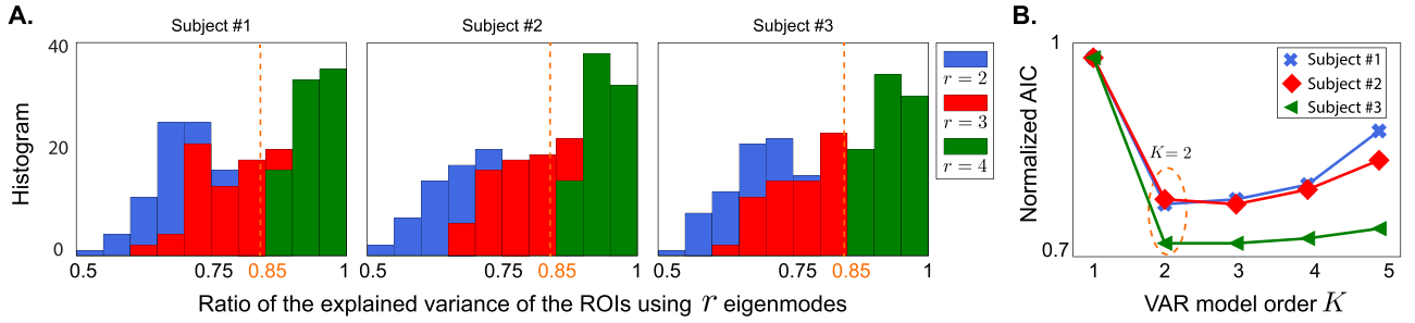
Fig. 10. Model selection curves. A. Histogram of the ratio of the explained variance to total variance for all ROIs using r = 2, 3, 4 eigenmodes for head models of three representative subjects. With r = 4 eigenmodes, at least 85% of the variance can be explained for all ROIs. B. AIC curve for r = 4 eigenmodes, suggesting a choice of K = 2 for the VAR model order for the three representative subjects.
