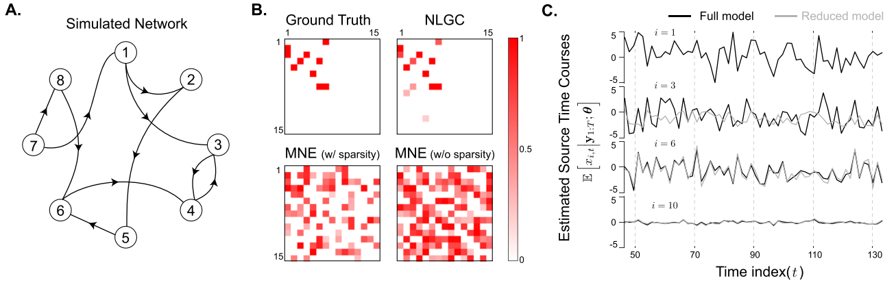
Fig. 2. An illustrative simulated example. A. The underlying true GC network between the active sources indexed by 1, 2, ..., 8 (explaining 90% of the power of the 84 sources). The remaining 76 sources are silent and are modeled as independent white noises accounting for the remaining 10% of the source power. B. The ground truth and estimated GC maps using NLGC and MNE (with and without accounting for sparsity). Only a subset of sources indexed by 1, 2, ..., 15 are shown for visual convenience. NLGC fully captures the true links with only a few false detection; on the other hand, the two-stage approaches using MNE, capture around half of the true links, but also detect numerous spurious links. While enforcing sparsity mildly mitigates the false alarm performance of the two-stage approach, it is unable to resolve it. C. Estimated activity time-courses of the patches with index 1, 3, 6, and 10 based on full models and the reduced models corresponding to the GC link ( 1 \mapsto 3 ) and non-GC links ( 1 \mapsto 6 ) and ( 1 \mapsto 10 ) as examples. As expected, since the GC link ( 1 \mapsto 3 ) exists, removing the 1st patch contribution from the VAR model of the 3rd patch dramatically changes the predicted activity of patch 3 (second line). However, this is not the case for the other two examples, since the links ( 1 \mapsto 6 ) and ( 1 \mapsto 10 ) do not exist (third and fourth lines).
