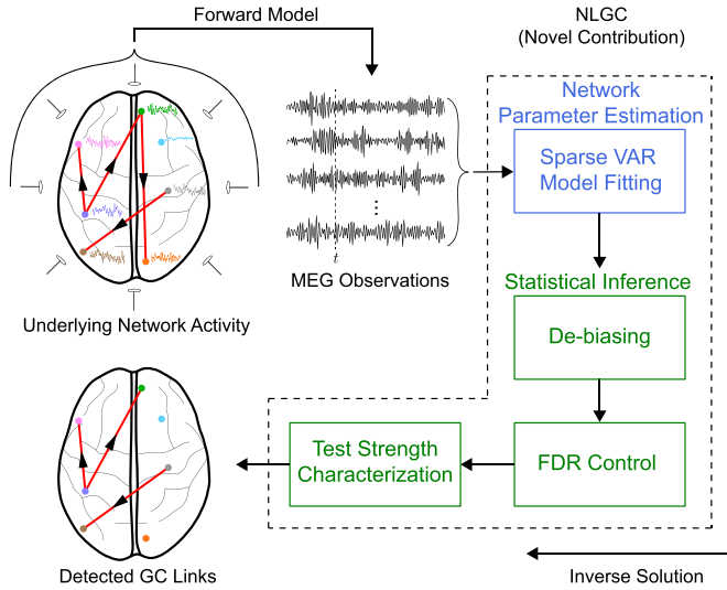
Fig. 1. A schematic depiction of the proposed NLGC inference. For cortical sources that form an underlying network, our contribution is to directly infer this network, using the framework of Granger, from the MEG measurements. NLGC is composed of network parameter estimation (blue block) and statistical inference (green blocks) modules. Unlike the conventional two-stage methods, NLGC extracts the GC links without an intermediate source localization step. (For interpretation of the references to color in this figure legend, the reader is referred to the web version of this article.)
