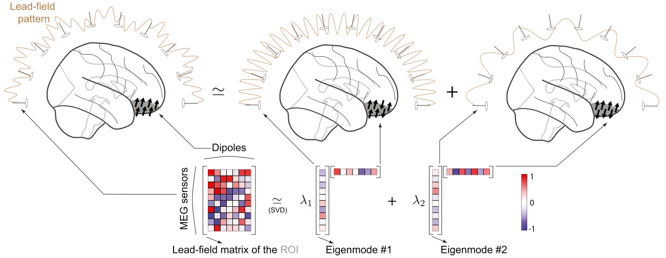
Fig. 9. An illustration of low-rank approximation to the lead-field matrix using eigenmode decomposition using r = 2 eigenmodes. The contribution of the 7 dipoles to 10 MEG sensors is originally captured by a 10 \times 7 sub-matrix of the lead-field matrix (left), whereas using the eigenmode decomposition, it can be approximated by two 10-dimensional eigenmodes (right), resulting in a 10 \times 2 effect sub-matrix.
